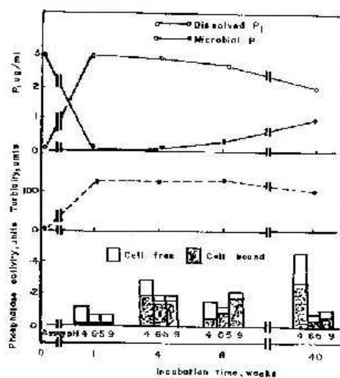
Figure 5b. Phosphatase activity, turbidity and microbial P_i of cultures of Awe cultivated soil micro-organism grown in P-limiting system.
