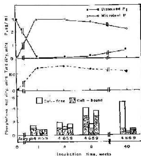
Figure 4a: Phosphatase activity, turbidity and microbial P of culture of the fallow soil micro-organism grown in P limiting system.
