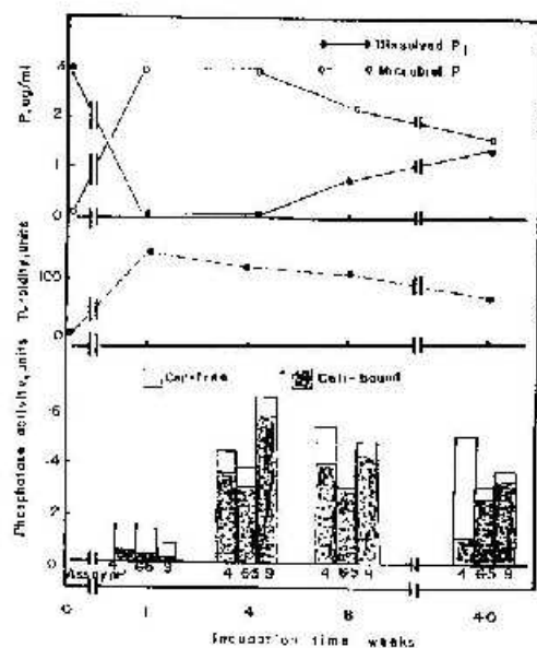
Figure 6b. Phosphatase activity, turbidity and microbial P of cultures of flora cultivated soil micro-organism grown in P limiting system.
